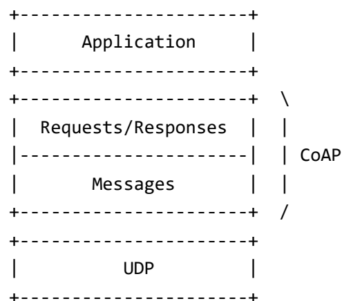
Figure 1: Abstract Layering of CoAP
