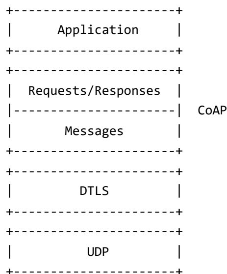
Figure 13: Abstract Layering of DTLS-Secured CoAP
