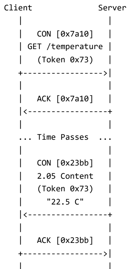
Figure 5: A GET Request with a Separate Response
