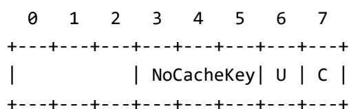
Figure 10: Option Number Mask (Least Significant Byte)
