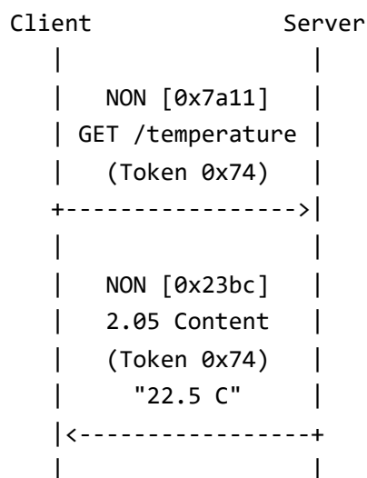
Figure 6: A Request and a Response Carried in Non-confirmable Messages
